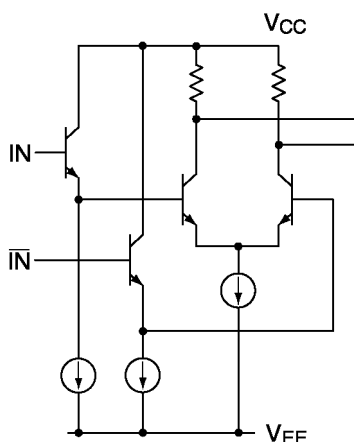
Figure 3. Simplified Input Buffer Schematic
