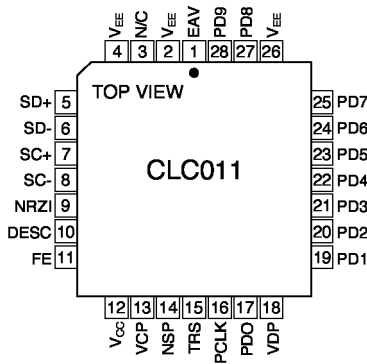
Figure 1. 28-Pin PLCC
