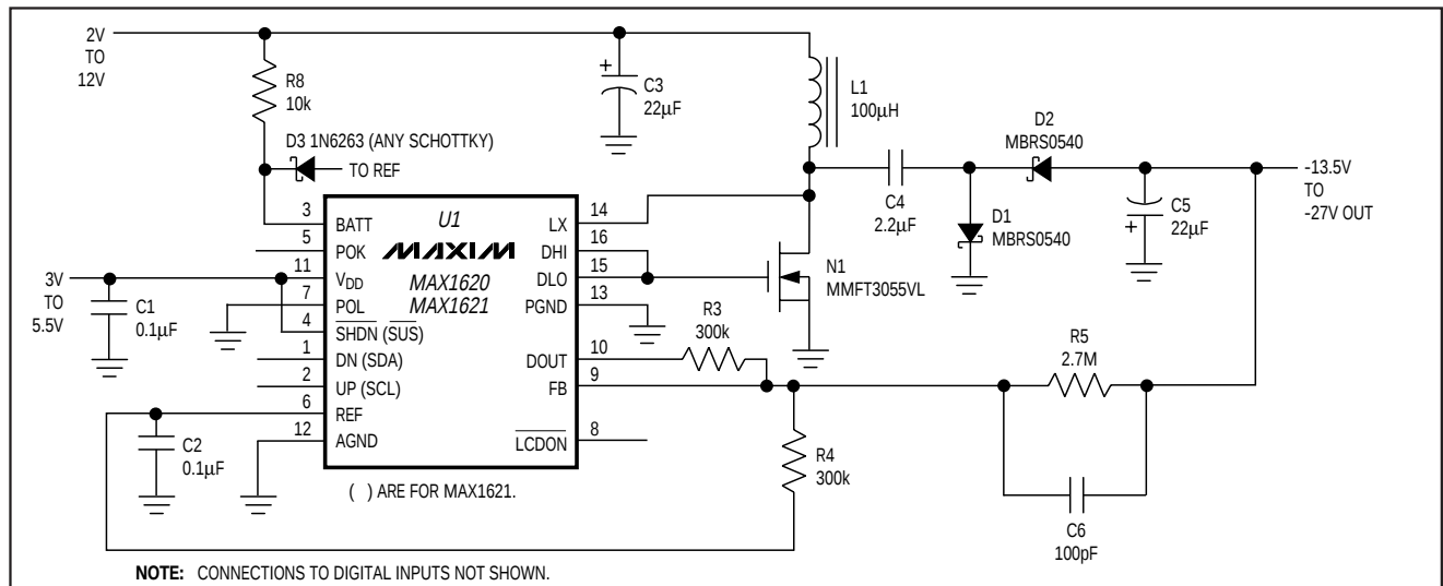
Figure 6. Alternative Negative Output—Maximum Voltage
