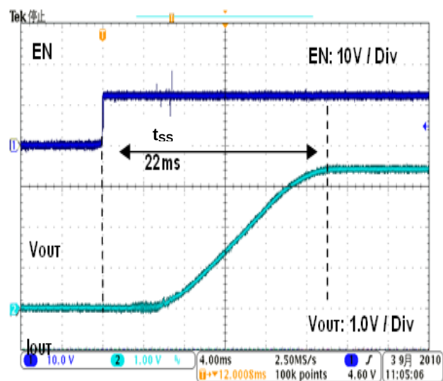
Figure 17. Start-Up Waveform ( V_{IN} = 12V V_{OUT} = 3.3V L = 10\mu H C_{SS} = 0.1\mu F )
