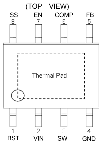
Figure 2. Pin Configuration
