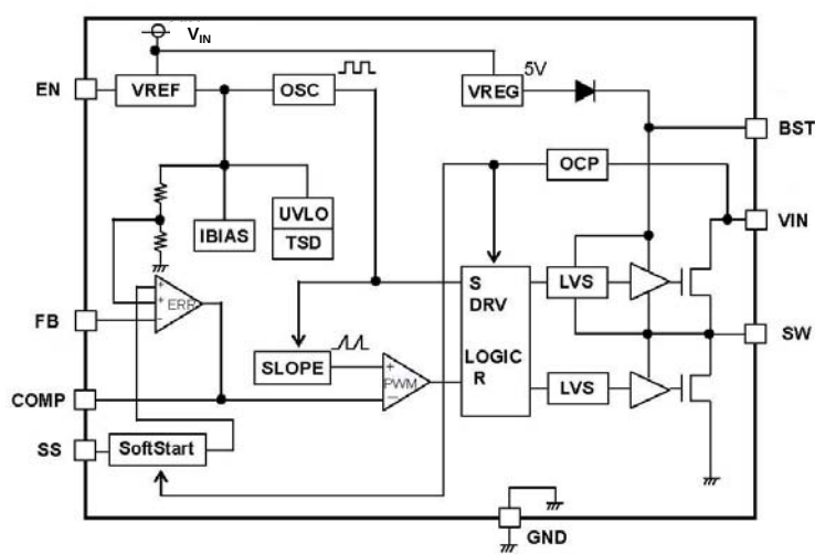
Figure 3. Block Diagram
