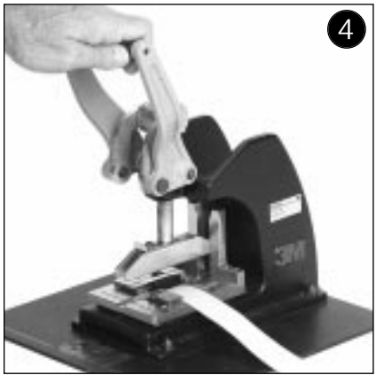
Lower the press handle to assemble the connector. It is recommended to check the tool setup before starting each production run. Proper seating of the connector cover onto the connector body can be checked by measuring the height of the connector/cover assembly.
