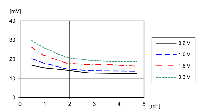
Output voltage ripple V_{pk-pk} at: T_{P1} = +25\text{ °C} , V_I = 12\text{ V} , I_O = 50\text{ A} . Parallel coupling of capacitors with 470 μF/10 mΩ
