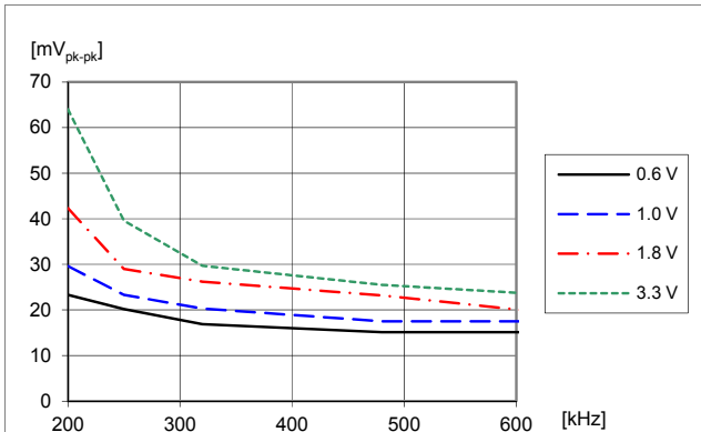
Output voltage ripple V_{pk-pk} at: T_{P1} = +25\text{ °C} , V_I = 12\text{ V} , C_O = 470\text{ μF}/10\text{ mΩ} , I_O = 50\text{ A} . Default configuration except changed frequency.
