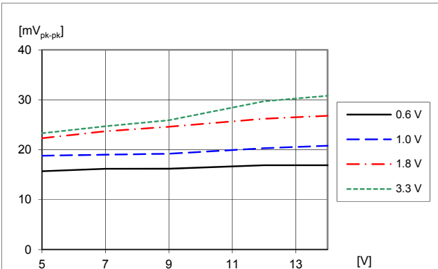
Output voltage ripple V_{pk-pk} at: T_{P1} = +25\text{ °C} , C_O = 470\text{ μF}/10\text{ mΩ} , I_O = 50\text{ A}
