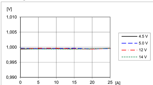
Load regulation at V_O = 1.0\text{ V} , T_{P1} = +25\text{ °C} , C_O = 470\text{ μF}/10\text{ mΩ}
