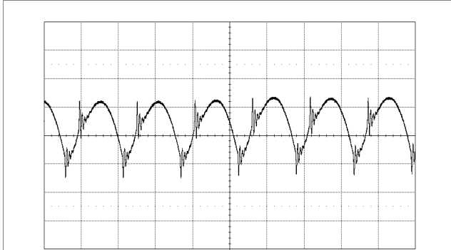
Output voltage ripple at: T_{P1} = +25\text{ °C} , Trace: output voltage (10 mV/div.). V_I = 12\text{ V} , C_O = 470\text{ μF}/10\text{ mΩ} Time scale: (2 μs/div.). I_O = 50\text{ A}
