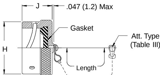
660-009 Receptacle Cover
