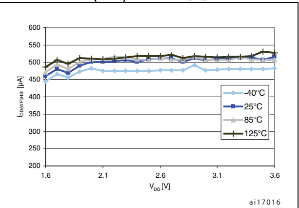
Figure 14. I_{DD(WAIT)} vs. V_{DD} , f_{CPU} = 16 \text{ MHz}
