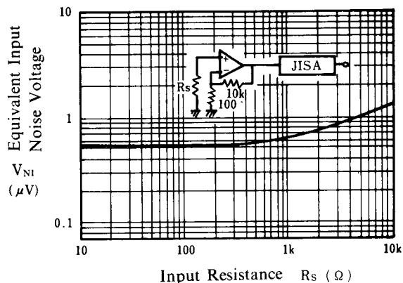
Equivalent Input Noise Voltage vs. Rs
