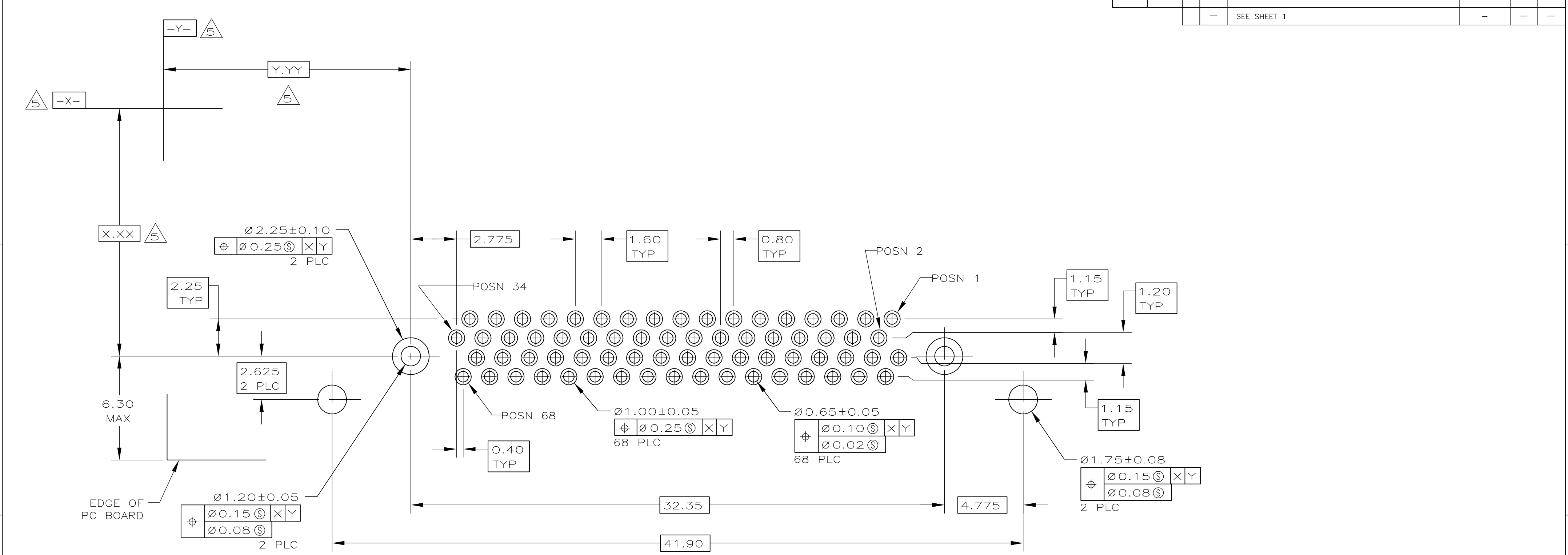
PC BOARD MOUNTING DIMENSIONS △3
