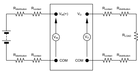
Figure 32. Output Ripple and Noise Test Setup.
