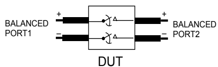
Diff. Insertion Loss and Return Test Circuit
