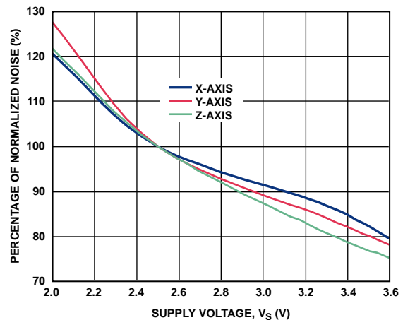
Figure 43. Normalized Noise vs. Supply Voltage, V_s
