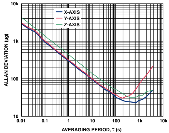
Figure 42. Root Allan Deviation
