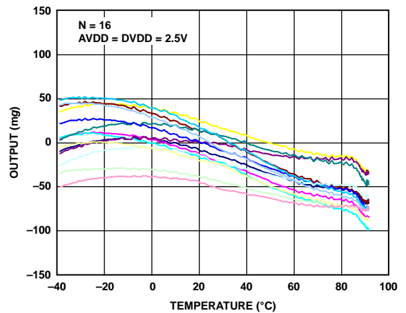
Figure 9. Z-Axis Zero g Offset vs. Temperature— Eight Parts Soldered to PCB, V_S = 2.5\text{ V}
