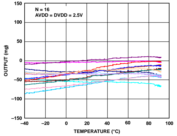
Figure 7. X-Axis Zero g Offset vs. Temperature— Eight Parts Soldered to PCB, V_S = 2.5\text{ V}
