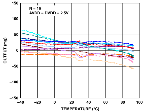
Figure 8. Y-Axis Zero g Offset vs. Temperature— Eight Parts Soldered to PCB, V_S = 2.5\text{ V}
