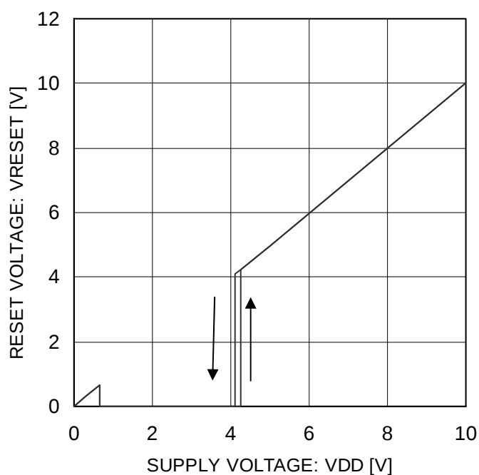
Figure 3. Detection Voltage
