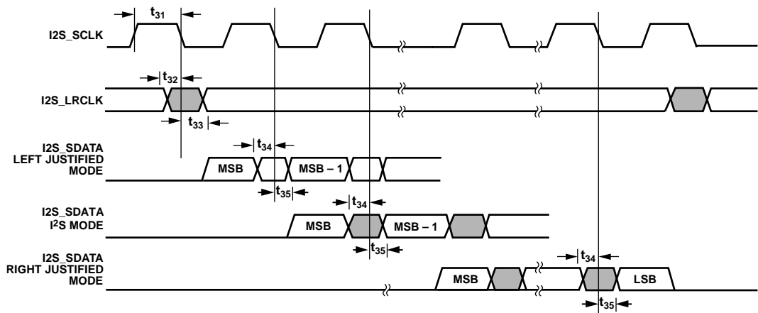
Figure 11. I 2 S Timing
