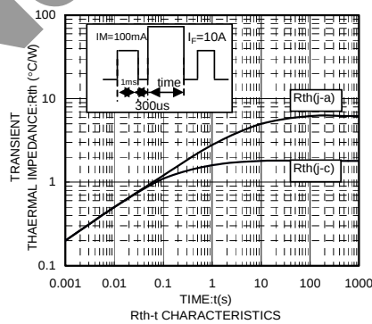
R_{\theta JA} - t CHARACTERISTICS
