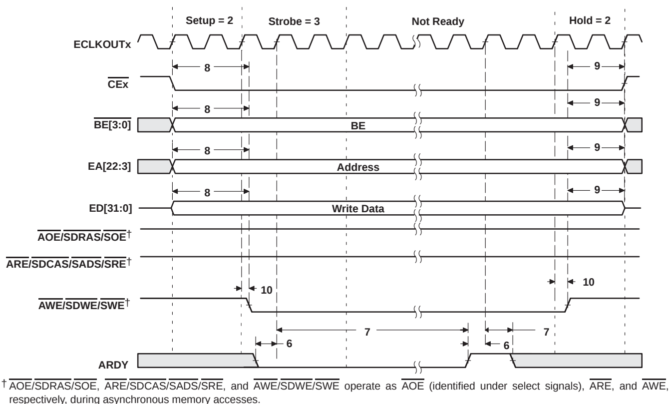
Figure 23. Asynchronous Memory Write Timing
