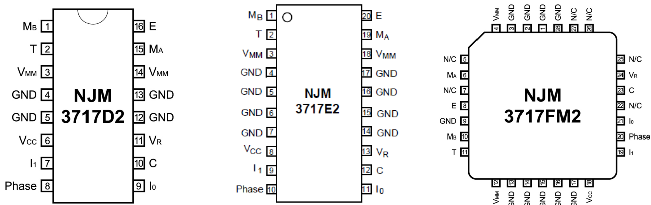
Figure 2. Pin configurations
