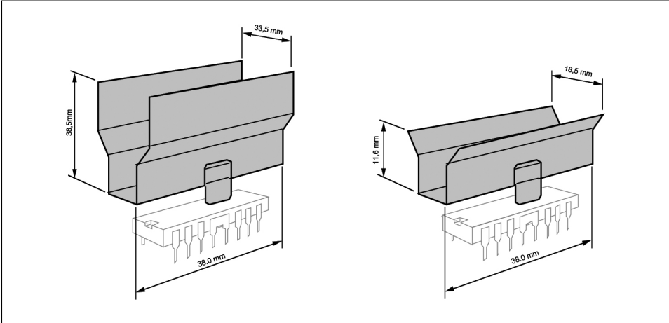
Figure 9. Heatsinks, Staver, type V7 and V8 by Columbia-Staver UK
