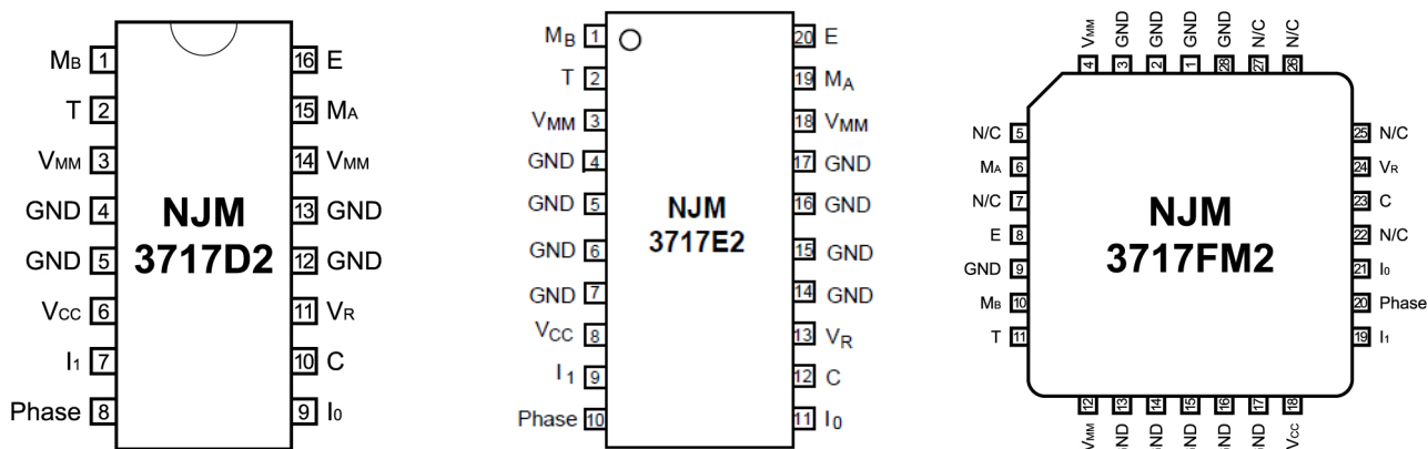
Figure 2. Pin configurations
