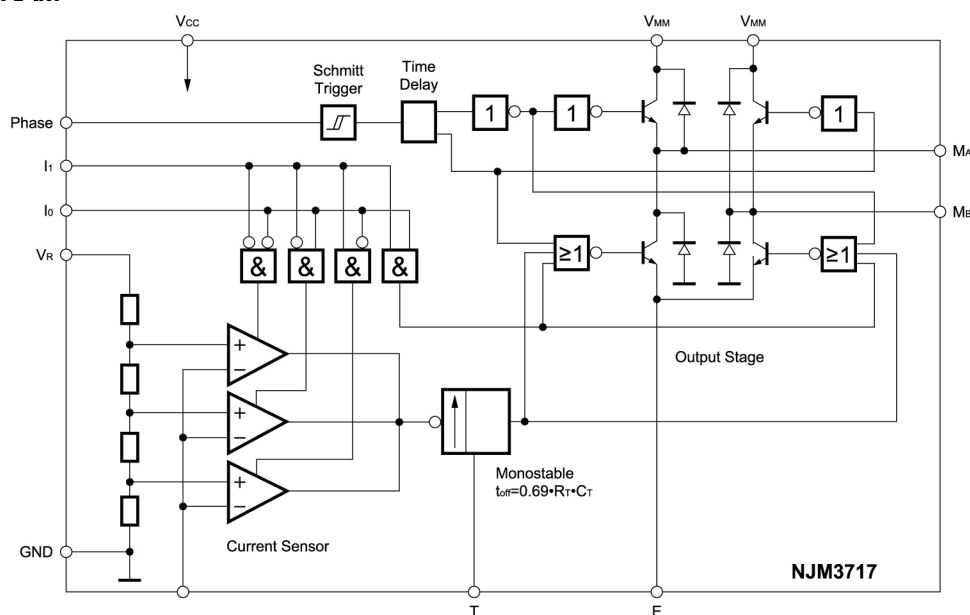
Figure 1. Block diagram
