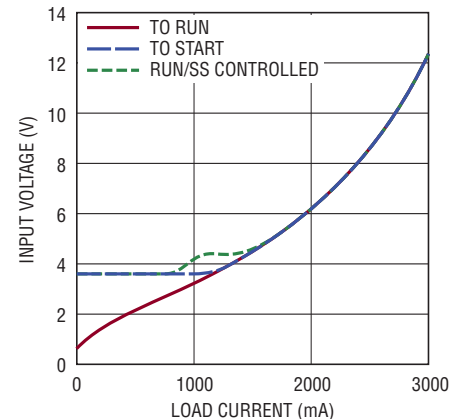
Minimum Input Voltage vs Load Current, -5V_{OUT}
