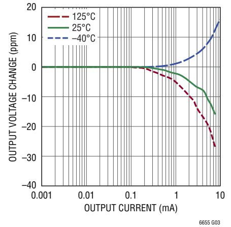
1.25V Sinking Current with a 3.3μF Output Capacitor
