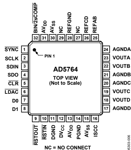
Figure 6. Pin Configuration
