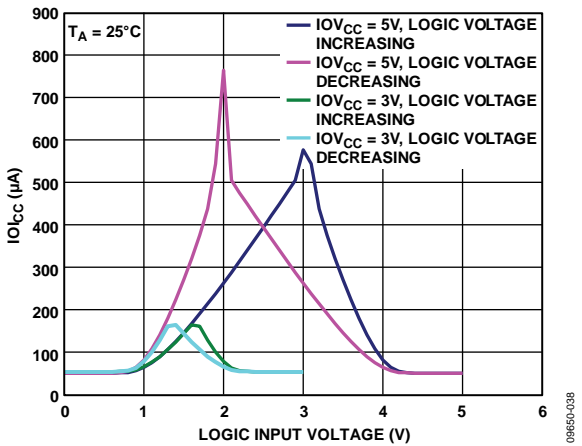
Figure 37. IO_{LCC} vs. Logic Input Voltage
