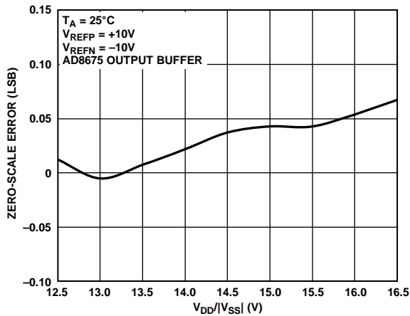
Figure 19. Zero-Scale Error vs. Supply Voltage, ±10 V Span
