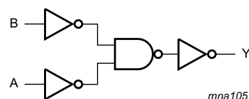
Fig 3. Logic diagram
