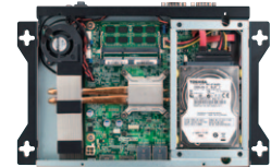
AIMB-B1230
