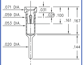
8855-0-15-XX-30-XX-34-0 Press-fit in .057 mounting hole
