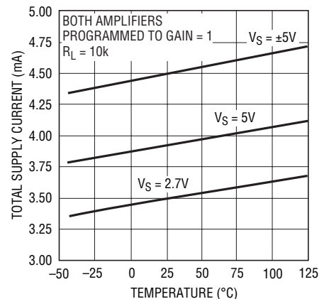
LTC6912-1 Total Supply Current vs Temperature (Both Amplifiers Active)
