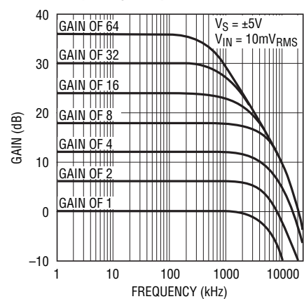
LTC6912-2 Frequency Response
