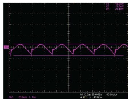
Figure 14. Output voltage ripple 230 V IN_AC full load
