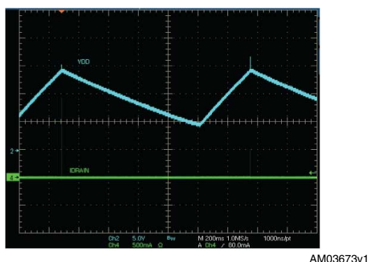
Figure 33. Operating with secondary winding shorted. Restart mode
