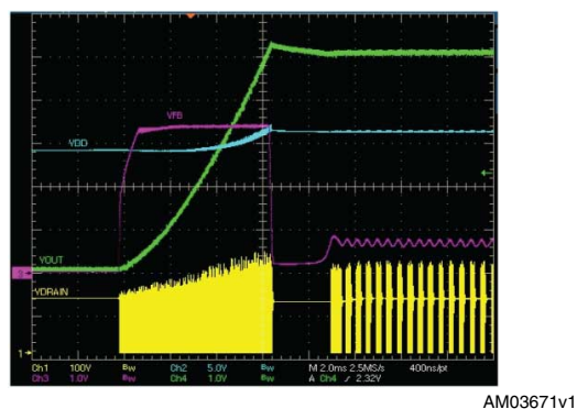
Figure 31. OLP: restart after short removal (zoom)
