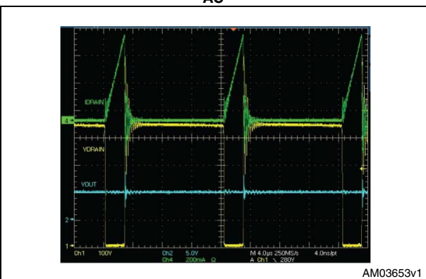
Figure 12. Drain current and voltage at peak load 265 V AC
