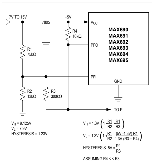
Figure 12. Adding Hysteresis to the Power-Fail Voltage Comparator
