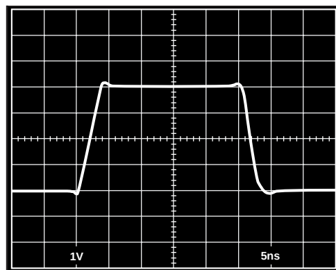
Figure 15. AD9632 Large Signal Transient Response; V_{OUT} = 4\text{ V p-p} , G = -1 , R_F = R_{IN} = 422\ \Omega , R_T = 56.2\ \Omega
