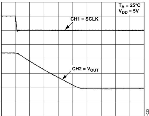
CH1 = 5V/DIV CH2 = 1V/DIV TIME BASE = 2 \mu s/DIV
