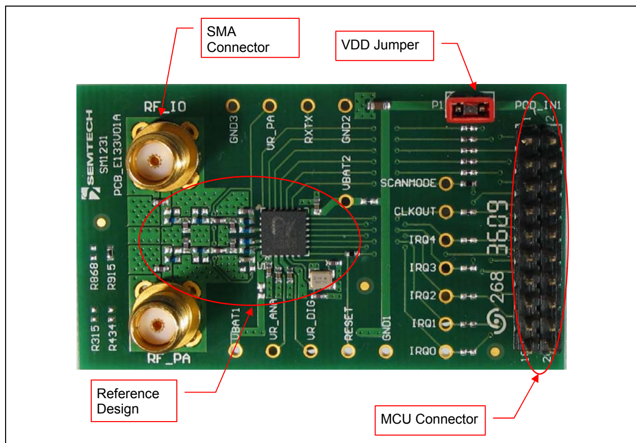
Figure 1: SM1211 Overview (Top View)
