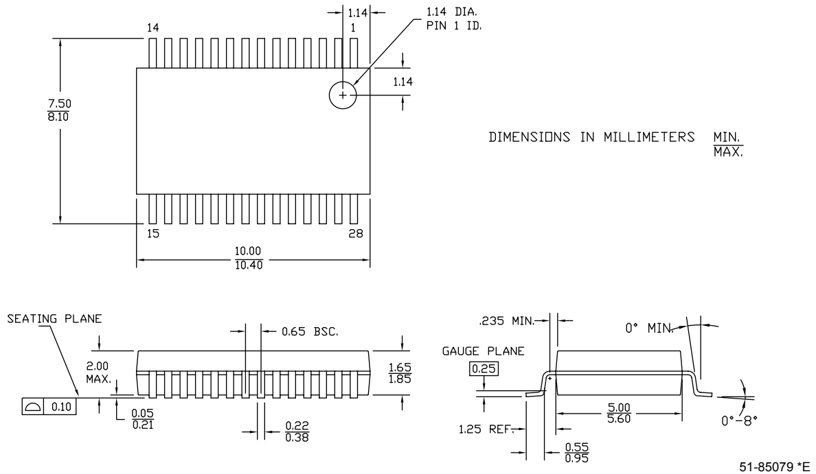
Figure 22. 28-Pin (210-Mil) SSOP
