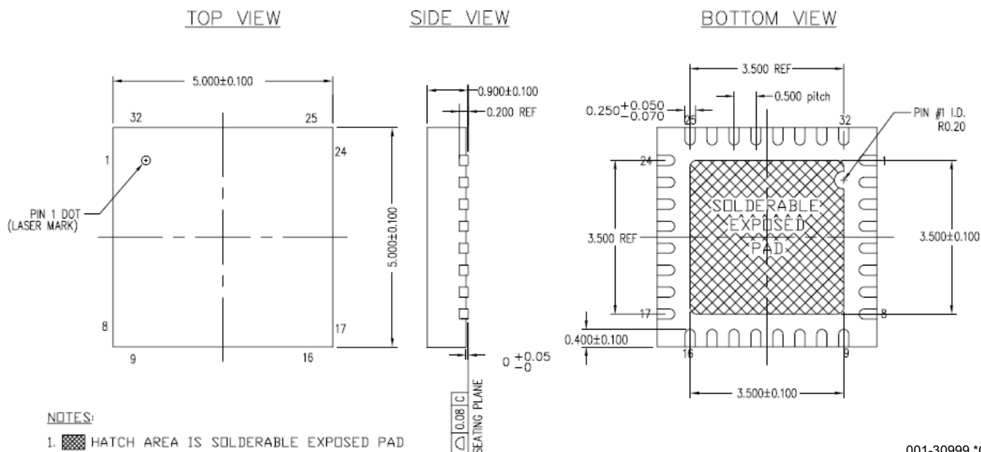
Figure 24. 32-Pin Sawn QFN Package
