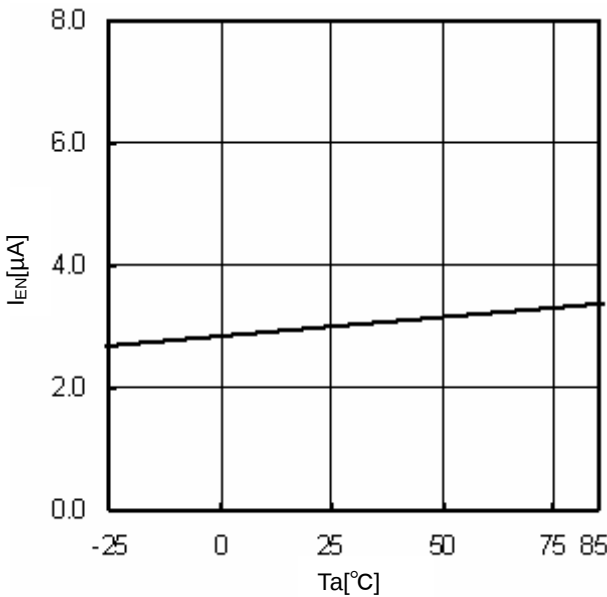
Fig.14 T_a - I_{EN}
