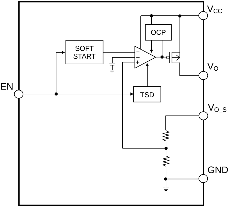
Fig.2 Block Diagram
