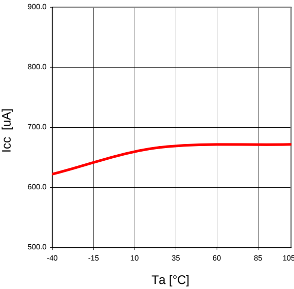
Figure 22. T_a - I_{cc}
