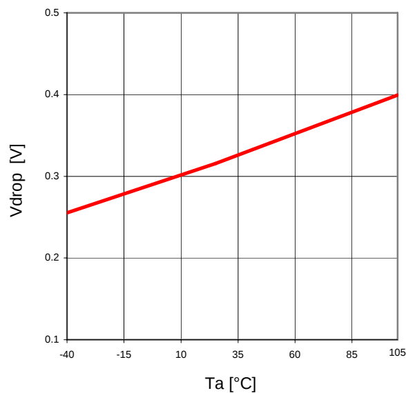
Figure 33. T_a - V_{drop} ( V_{CC}=6\text{V} , I_o=0.3\text{A} )
