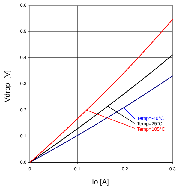
Figure 34. Minimum dropout Voltage 1 ( V_{CC}=4.5\text{V} )
