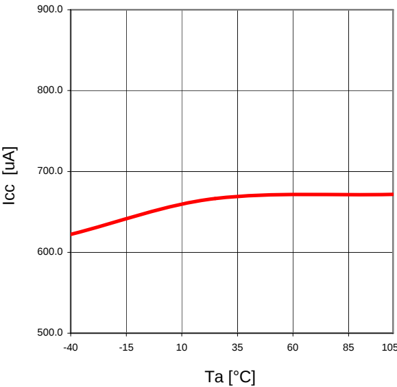
Figure 22. T_a - I_{cc}
