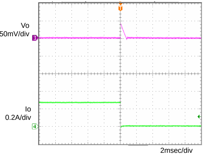
Figure 6. Transient Response (0.3→0A) Co=1 \mu F, Ta=-40°C
