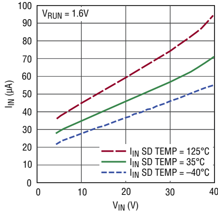
IN Pin Disabled Current vs Input Voltage
