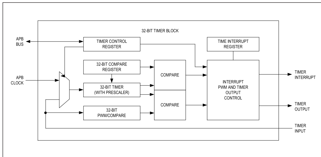
Figure 3. 32-Bit Timer
