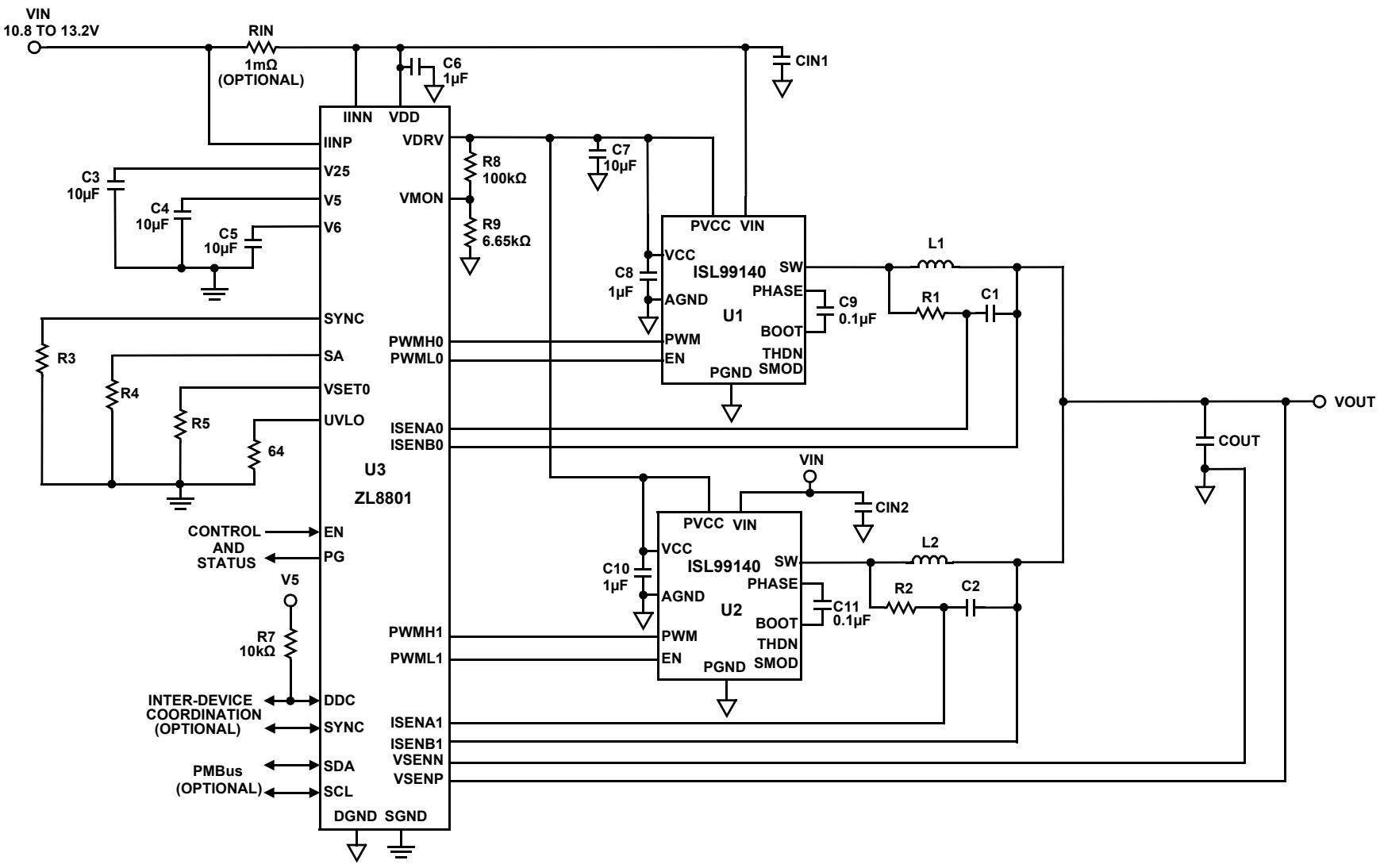
FIGURE 3. ZL8801 SCHEMATIC
