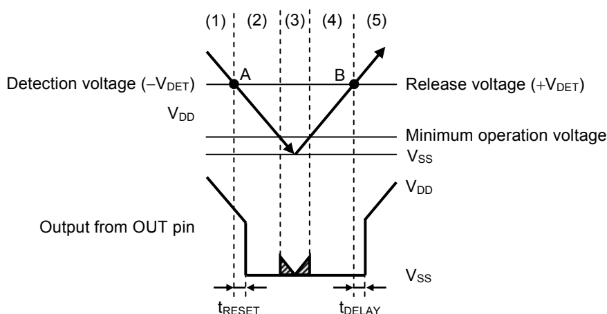
Figure 25 Operation of S-1011 Series C / L Type
