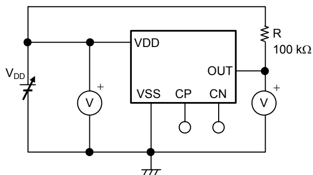
Figure 7 Test Circuit 1 (VDD detection product)
