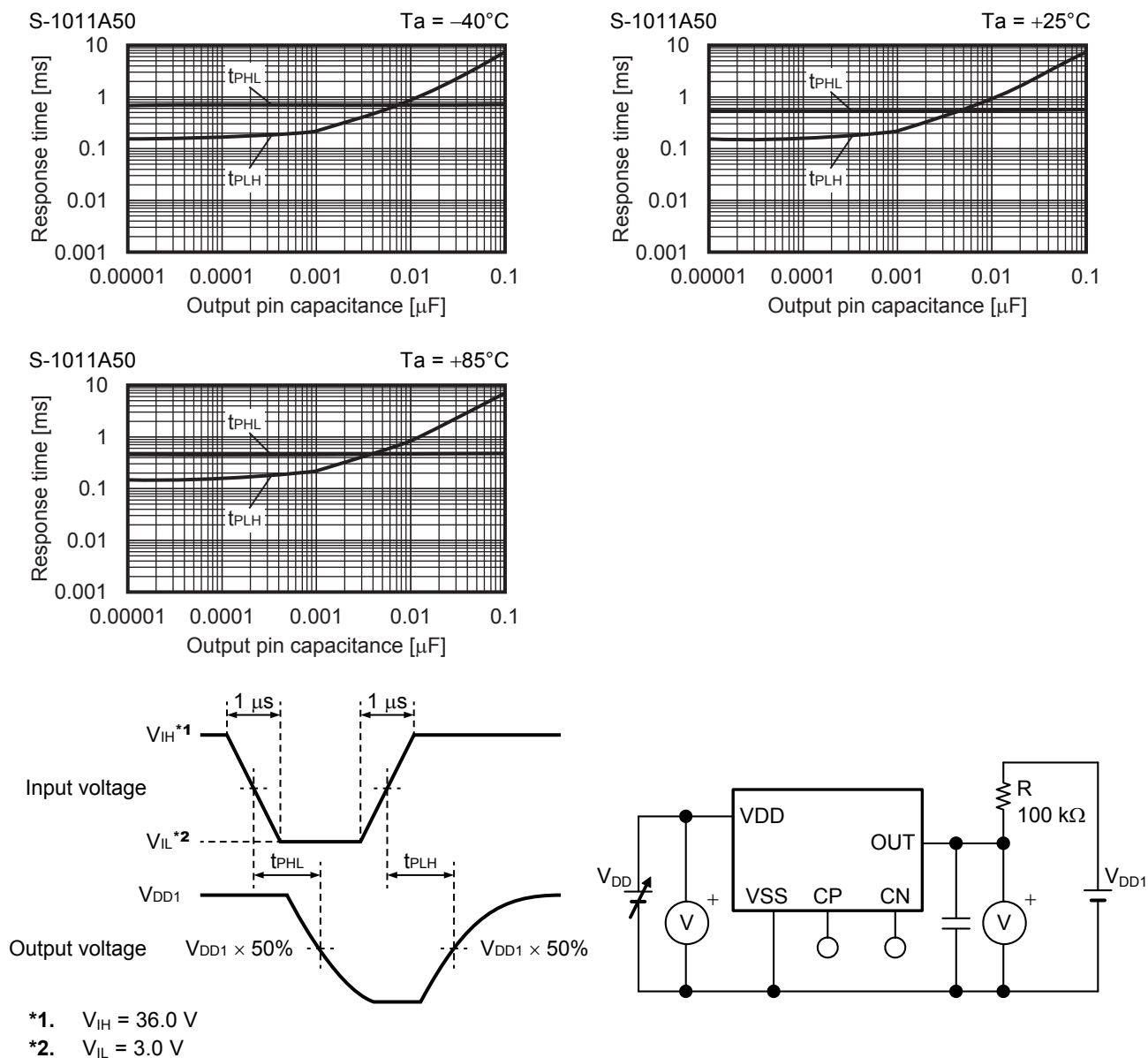
Figure 43 Test Condition of Response Time
