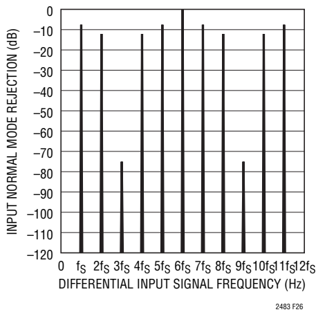
Figure 26. Input Normal Mode Rejection, External Oscillator ( f_{\text{EOSC}} = 256\text{kHz} ) 50Hz Rejection
