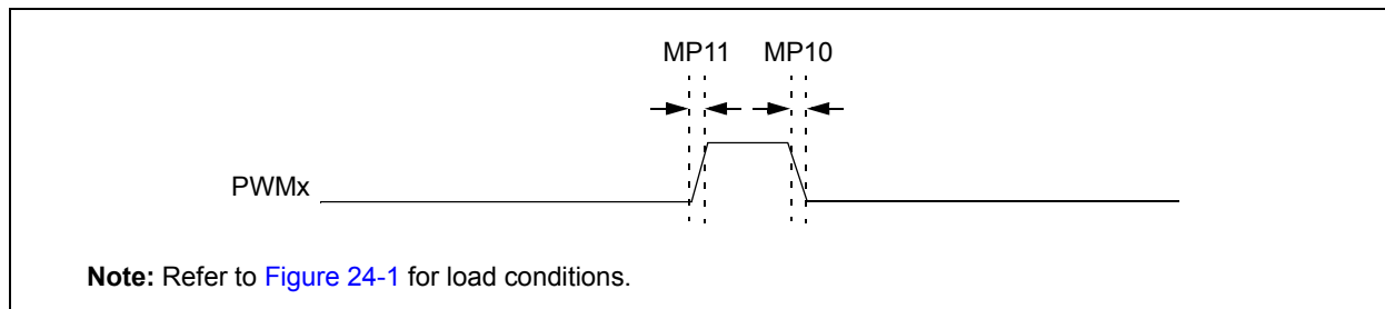
FIGURE 24-6: HIGH-SPEED PWMx MODULE TIMING CHARACTERISTICS
