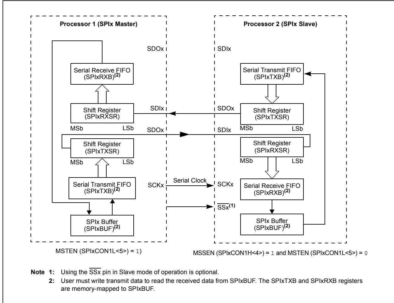
FIGURE 14-4: SPIx MASTER/SLAVE CONNECTION (ENHANCED BUFFER MODES)
