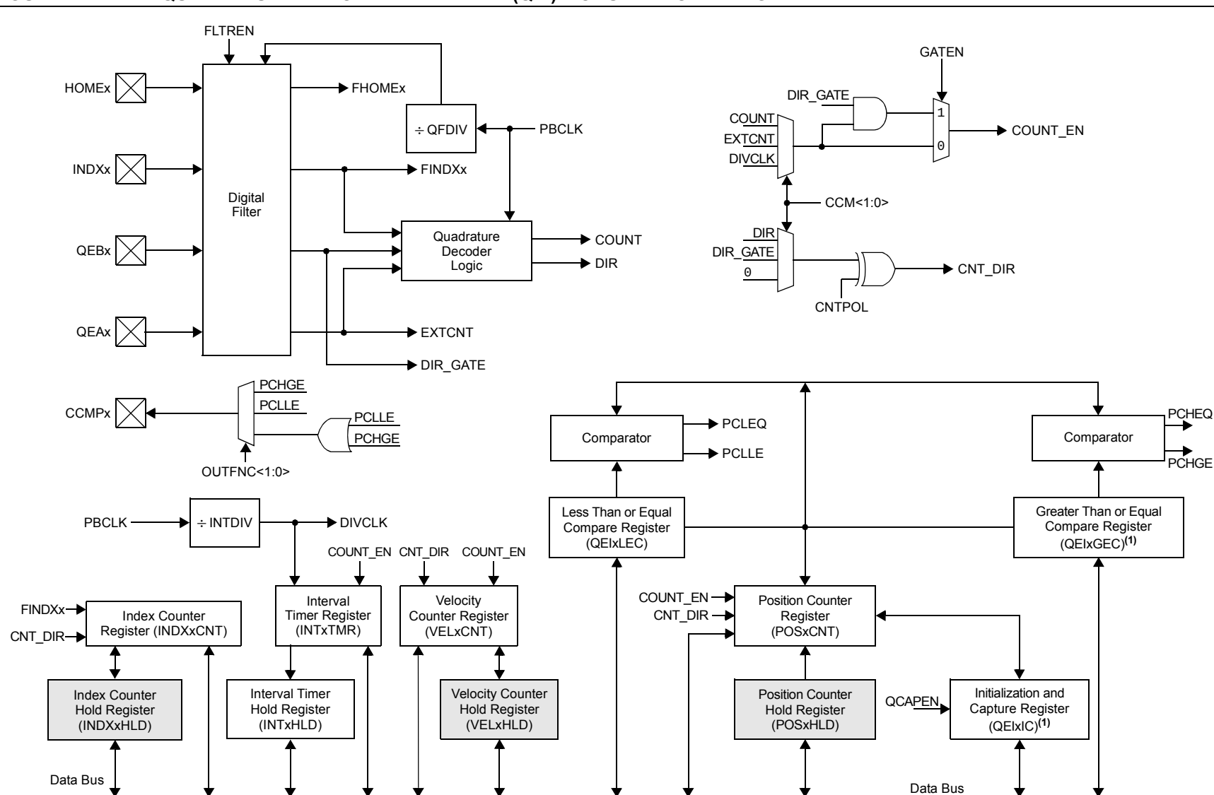
FIGURE 12-2: QUADRATURE ENCODER INTERFACE (QEI) MODULE BLOCK DIAGRAM
