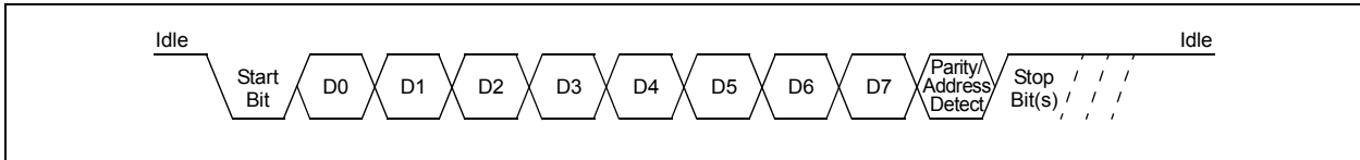
FIGURE 13-2: UART CHARACTER FRAME
