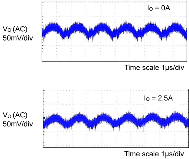
Figure 18. Output Voltage Ripple Wave V_{IN} = 24V, V_O = 5.0V
